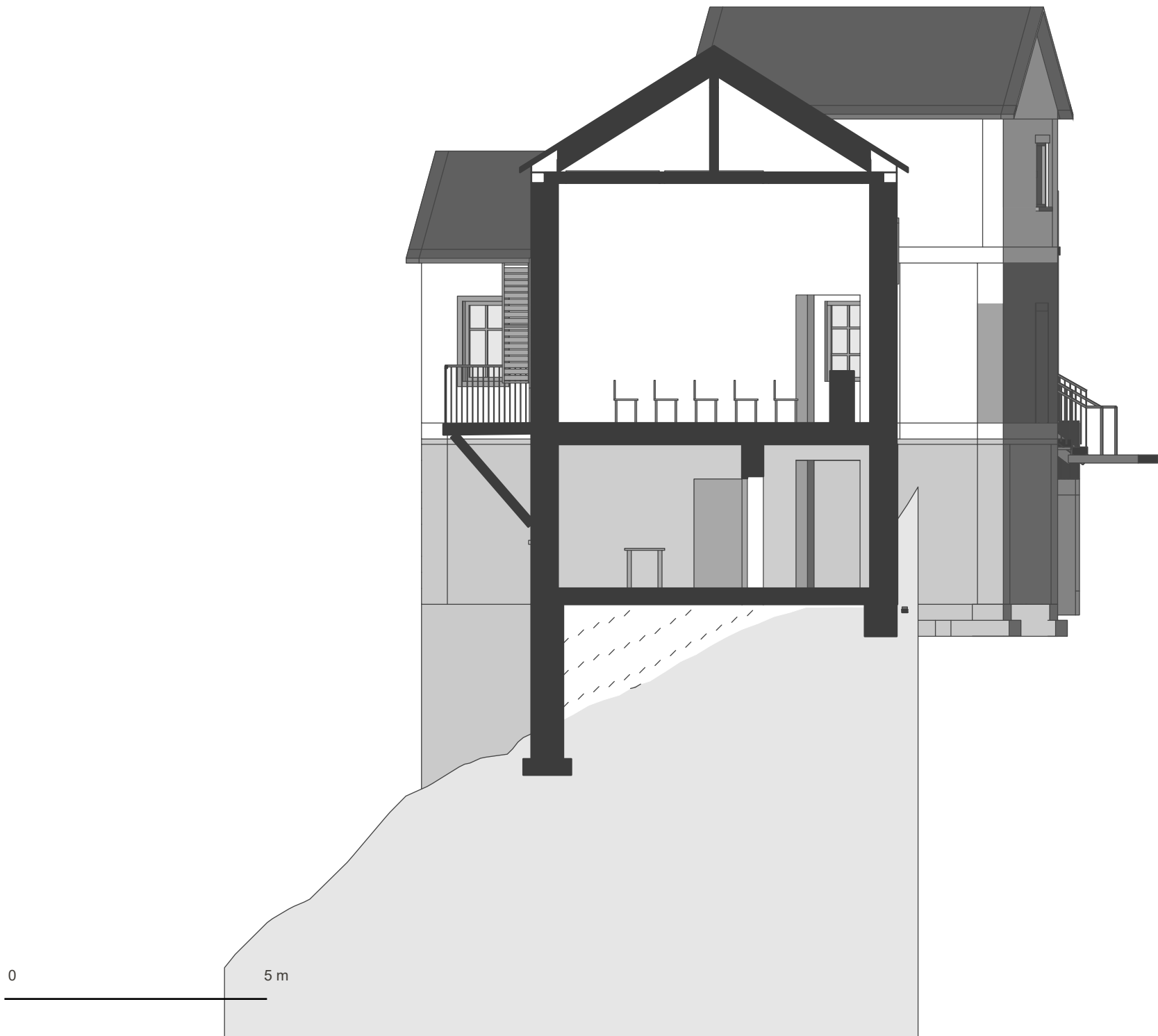
TRUE TRANSVERSE / HALL X=191 in | Gable and existing trusses above flat opaque coffered ceiling.
