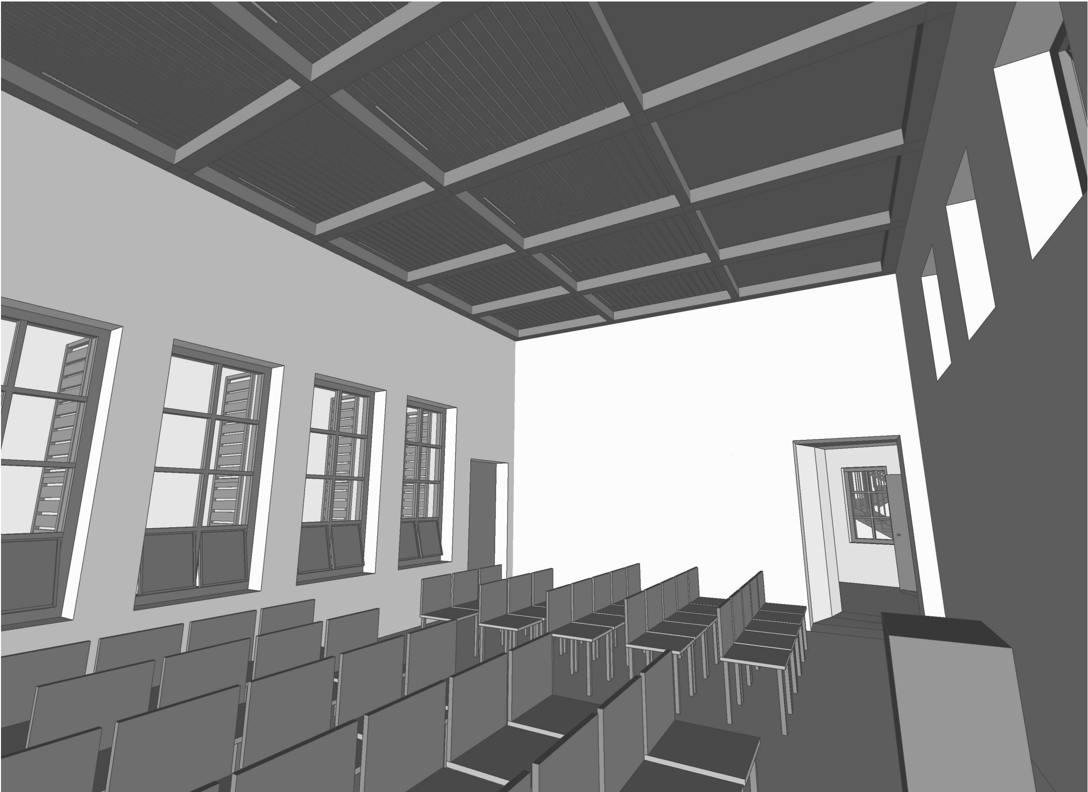
Actual flat opaque coffered ceiling below retained gable/truss roof; twelve absorption zones and six reflection zones, performance untested.
